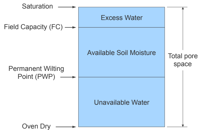
Figure 1. The various levels of the soil water content.
