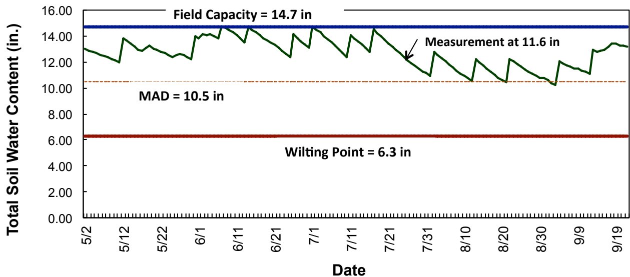
Figure 3. Soil water contents over time from the above examples (1 and 2).
